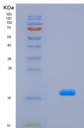
Figure . SDS-PAGE
