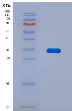
Figure 1. SDS-PAGE
