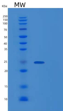
Figure 1. SDS-PAGE
