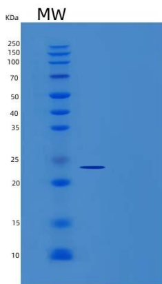
Figure 1. SDS-PAGE
