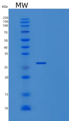
Figure 1. SDS-PAGE
