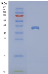
Figure 1. SDS-PAGE
