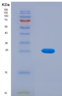
Figure 1. SDS-PAGE
